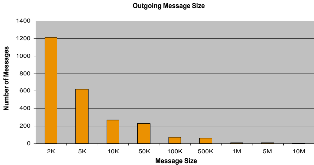
Figure 2 - Outgoing message breakdown
