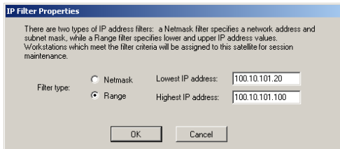
Fig. A-36 IP Filter Properties dialog box, Range
