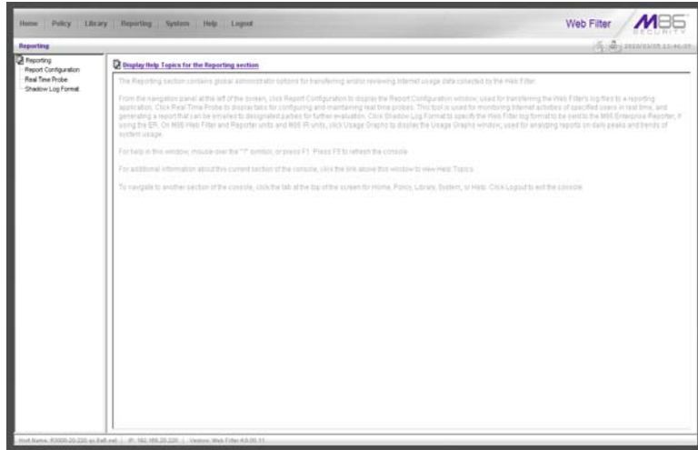
Fig. 2:4-1 Reporting screen
