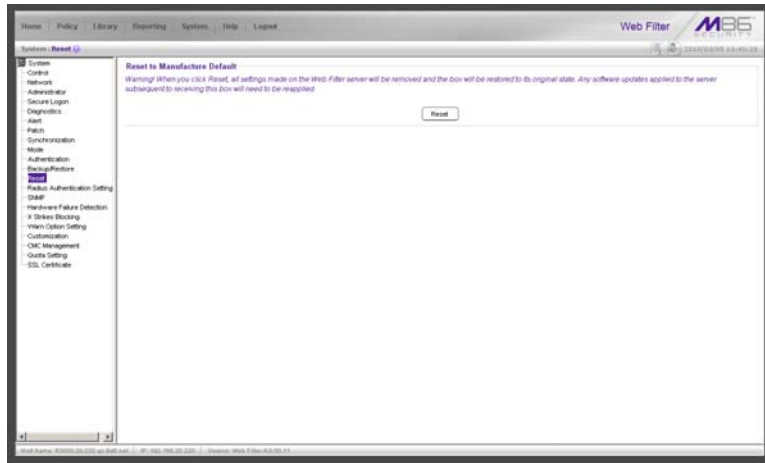
Fig. 2:1-58 Reset window
