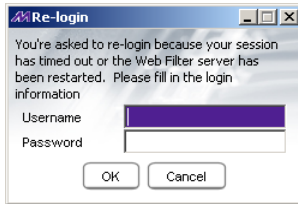
Fig. 2:1-68 Re-login window
