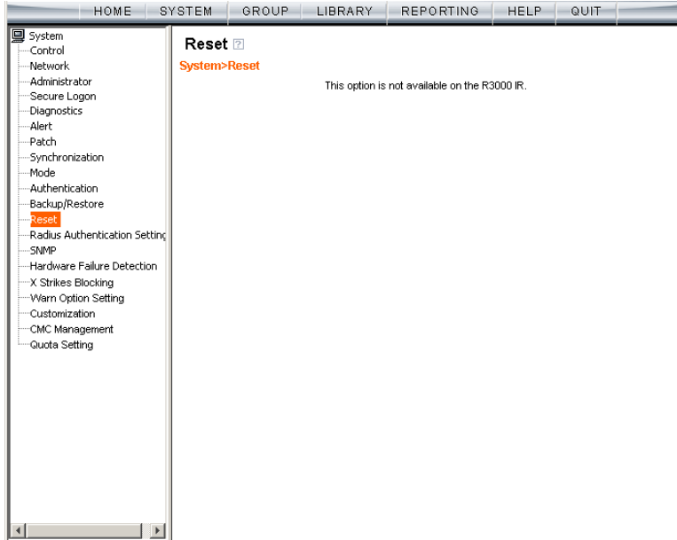
Fig. 2:1-78 Reset window
