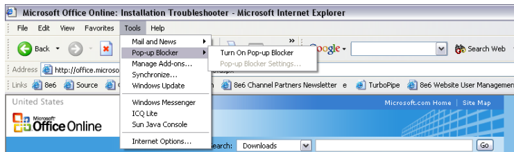
Fig. C-8 Toolbar setup
