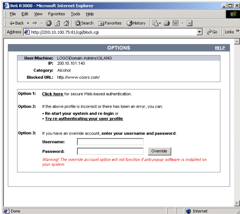
Fig. 2:1-6 Options page
