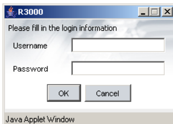
Fig. 2:1-88 Re-login window
