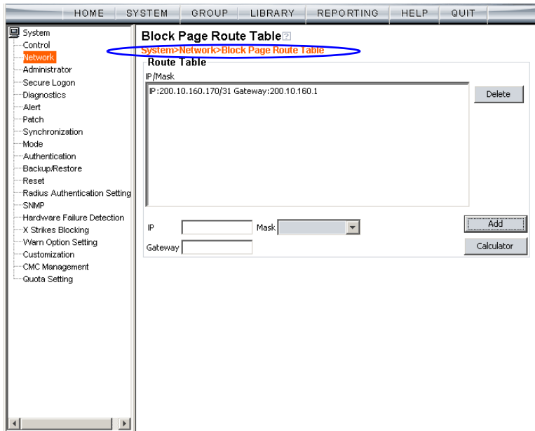
Fig. 1:4-14 Navigation path
