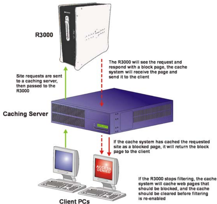
Fig. 1:1-5 Firewall mode diagram, with filtering and cache setup
