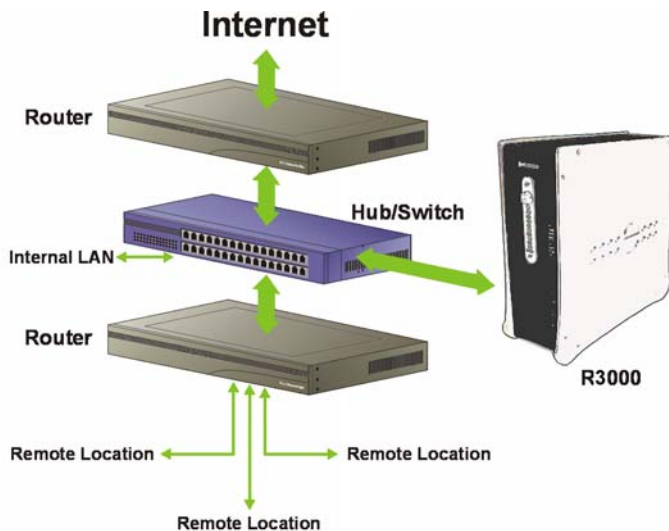
Fig. 1:1-3 Router mode diagram
